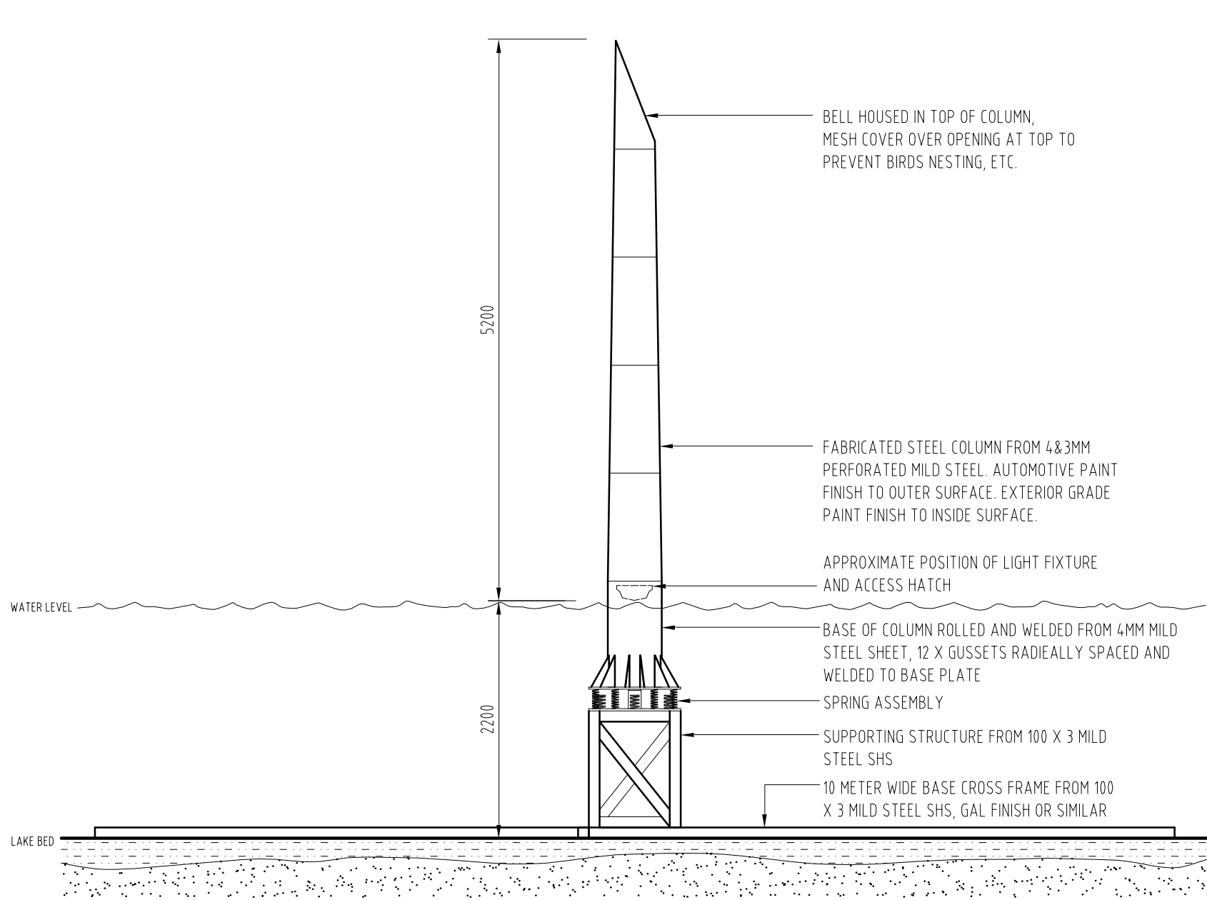
01 ELEVATION ASSEMBLED MODULE 1:50
