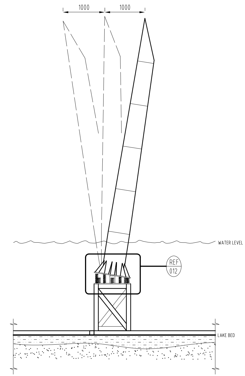
02 ELEVATION SHOWING DESIRED MOVEMENT 1:50
